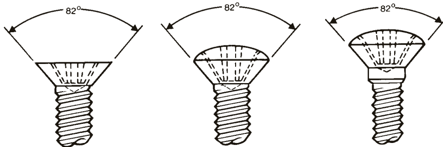
Phillips Flat Trim Heads 82°
